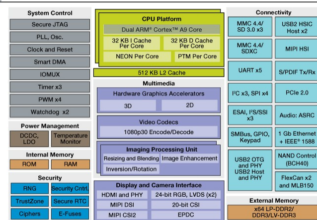
i.MX 6DualLite Multimedia Processor Block Diagram
