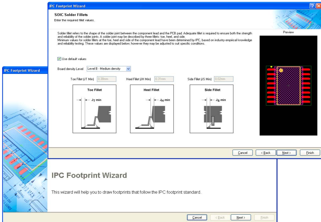
Figure 8. Quickly create IPC-compliant component footprints based on component dimensions in the new IPC Footprint Wizard .
