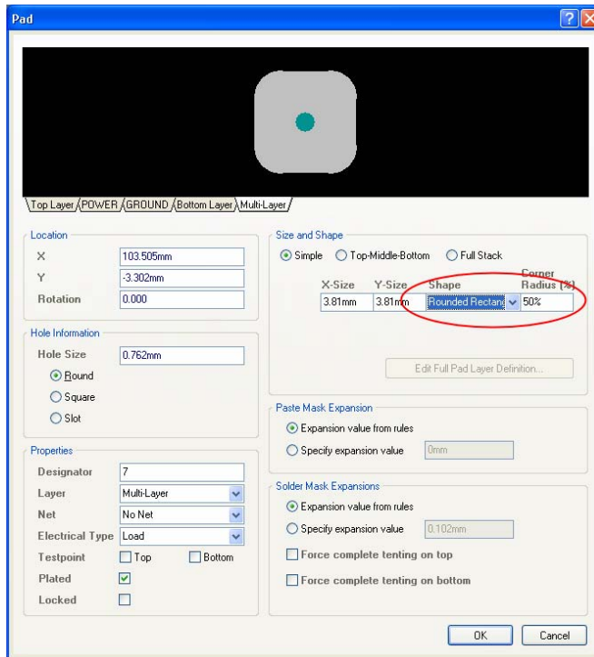
Figure 4. Create Rounded Rectangle pad shapes in your PCB.
