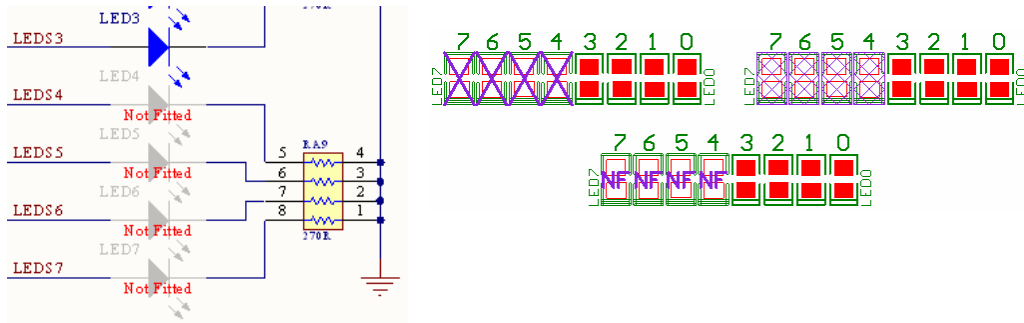
Figure 1. New options for handling schematic and PCB variant printing.
