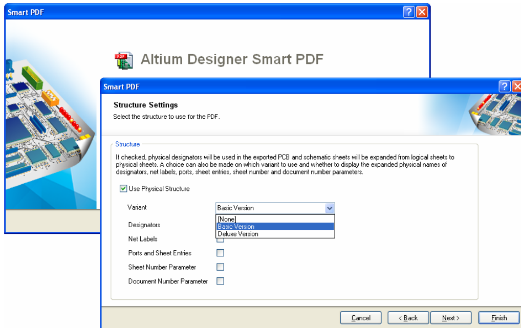
Figure 2. Specifying use of an assembly variant as part of the Smart PDF setup options.
