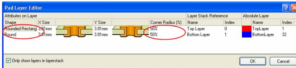
Figure 5. Define your pad size and shape for each layer in the pad stack, on a layer-by-layer basis.
