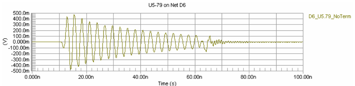
Figure 10. Experiment with Slew and Drive settings through the FPGA Signal Manager to see the effect on crosstalk.
