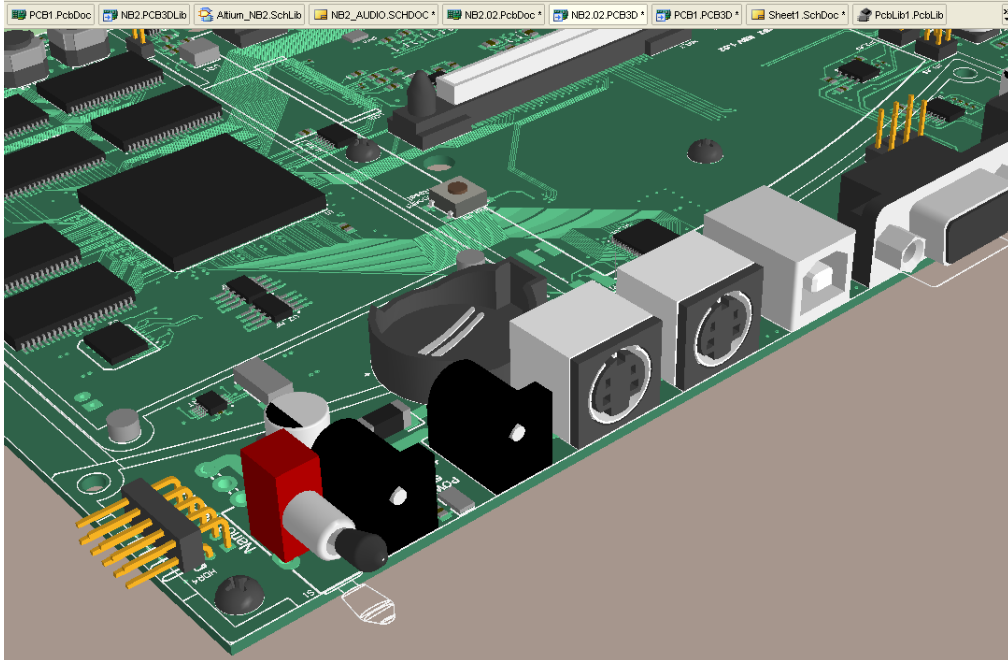
Figure 6. Once imported and associated to components, 3D STEP format models allow accurate representations of PCB boards to be created and transferred to Mechanical CAD applications.
