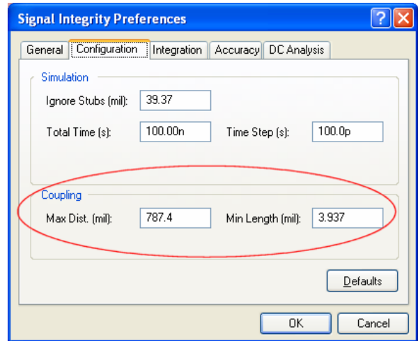
Figure 9. Set criteria to identify coupled nets.
