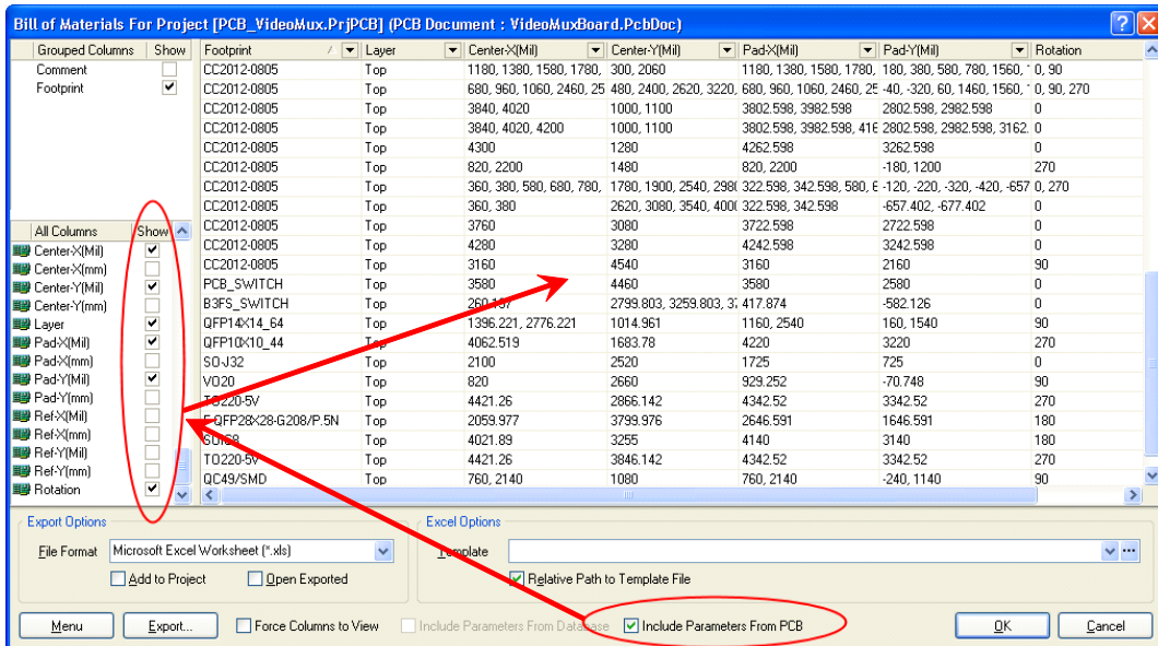
Figure 11. When configuring the Bill of Materials report using the Report Manager dialog, simply enable the Include Parameters From PCB option. This option will only be available if there is a PCB document in the project file.
